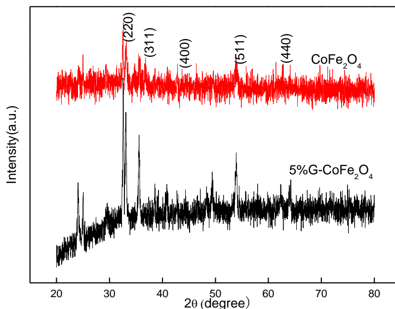
Fig-1: The typical XRD patterns of pure CoFe 2 O 4 and 5%G-CoFe 2 O 4 prepared at 180°C for 12h
