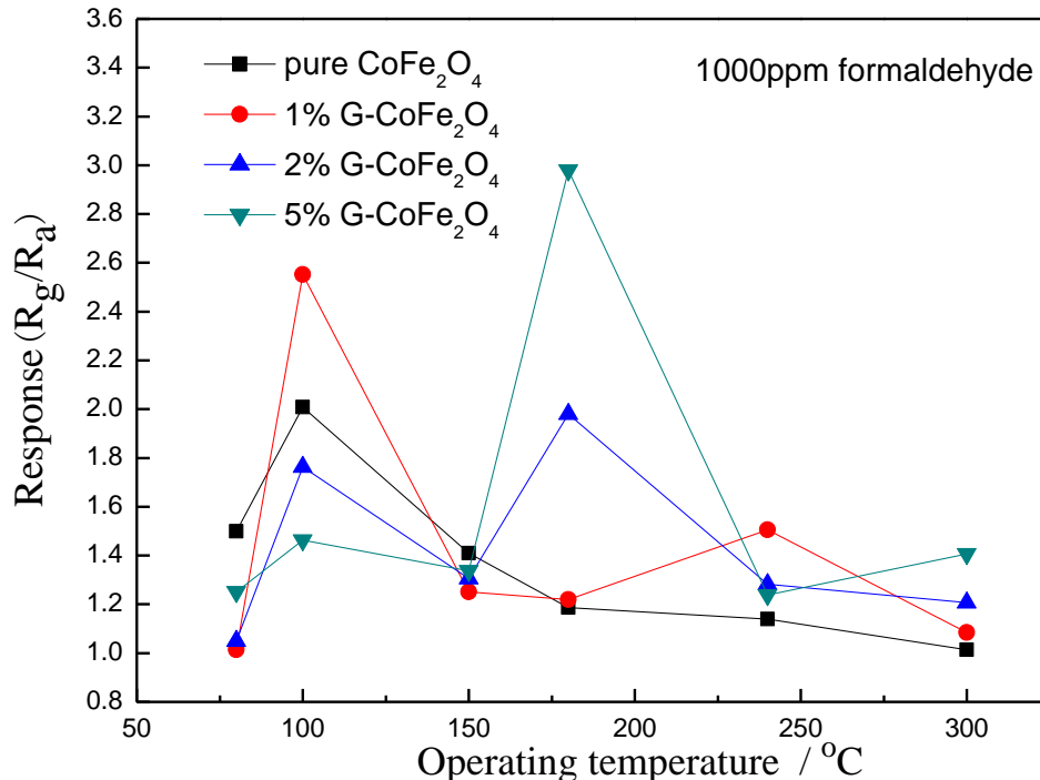
Fig-5: The responses to formaldehyde (1000 ppm) of sensors based on pure CoFe 2 O 4 and G-CoFe 2 O 4 (180°C, 12 h) with different mixing ratio
