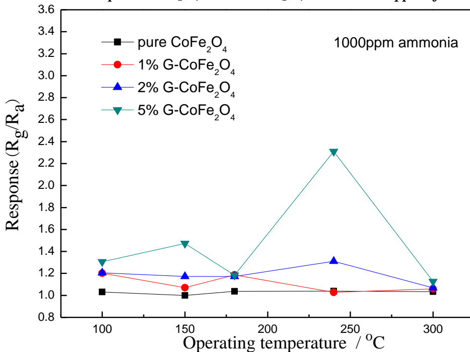
Fig-3: The responses to ammonia (1000 ppm) of sensors based on pure \text{CoFe}_2\text{O}_4 and G- \text{CoFe}_2\text{O}_4 (180°C, 12 h) with different mixing ratio
