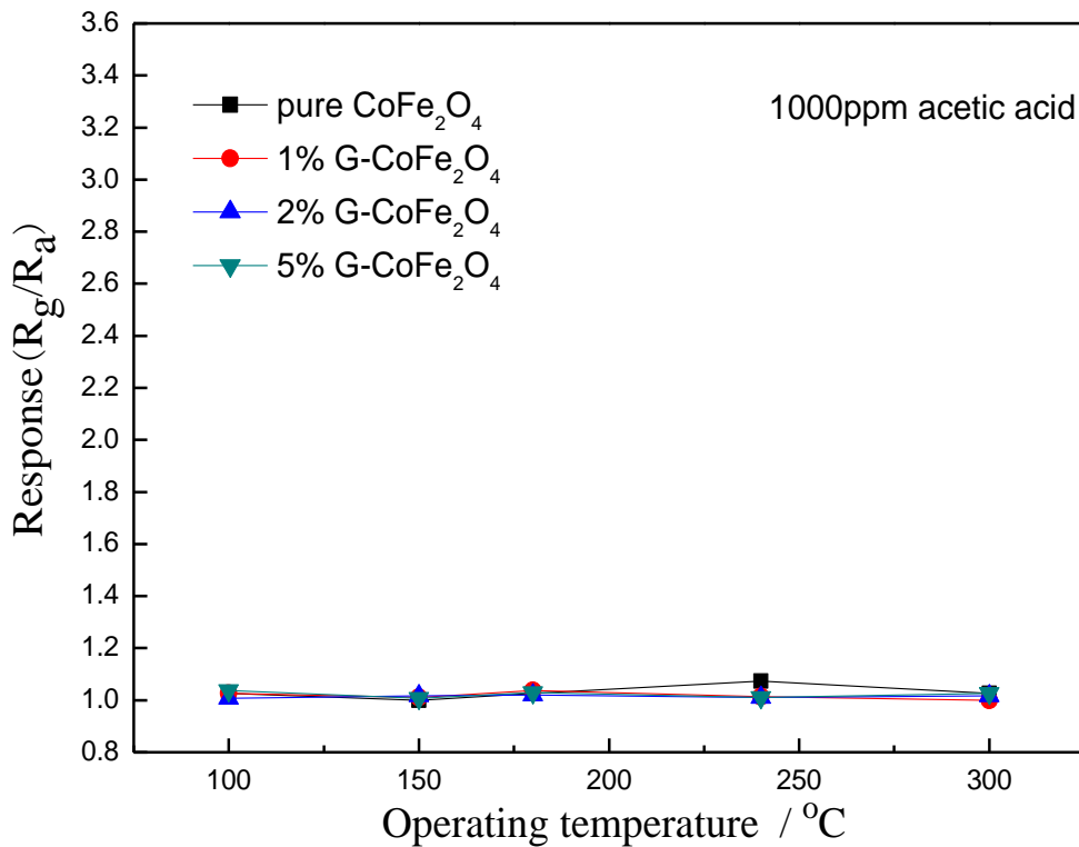
Fig-8: The responses to acetic acid (1000 ppm) of sensors based on pure \text{CoFe}_2\text{O}_4 and G- \text{CoFe}_2\text{O}_4 (180 ^{\circ}\text{C} , 12h) with different mixing ratio
