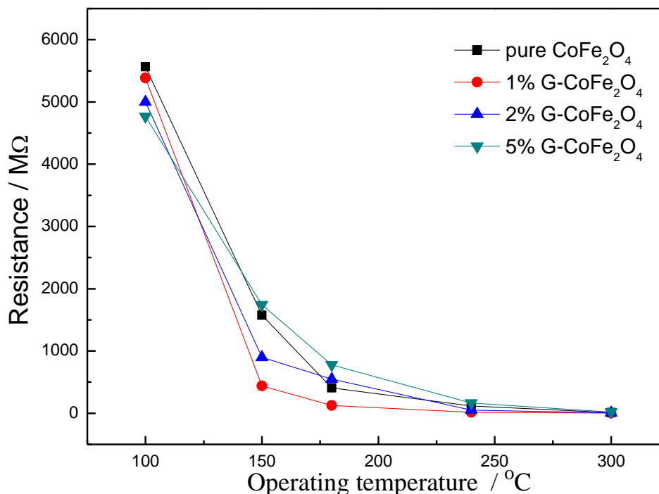
Fig-9: The electrical resistances of pure \text{CoFe}_2\text{O}_4 sensor and G- \text{CoFe}_2\text{O}_4 sensors in air at different operating temperatures
