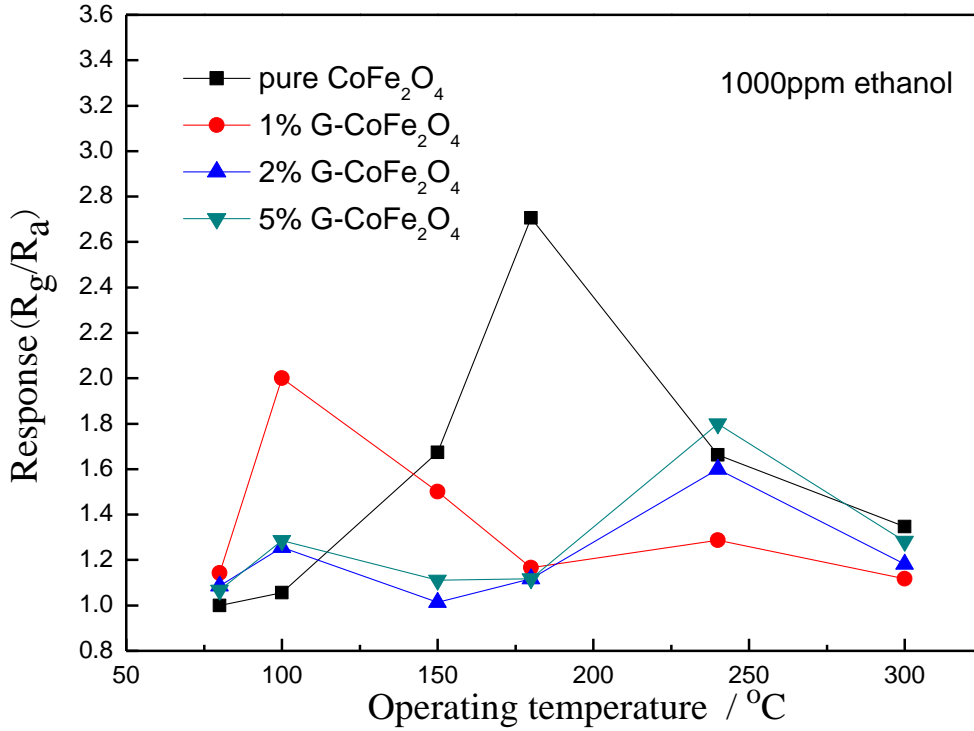
Fig-6: The responses to ethanol (1000 ppm) of sensors based on pure CoFe 2 O 4 and G-CoFe 2 O 4 (180°C, 12h) with different mixing ratio
