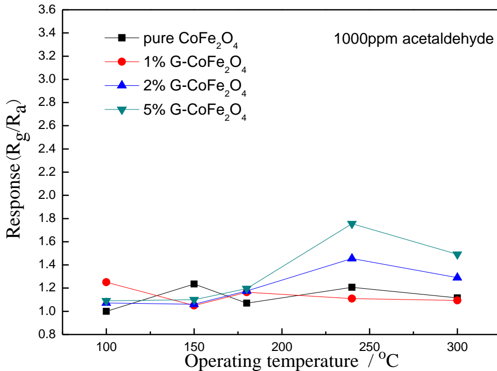
Fig-7: The responses to acetaldehyde (1000 ppm) of sensors based on pure CoFe 2 O 4 and G-CoFe 2 O 4 (180°C, 12 h) with different mixing ratio
