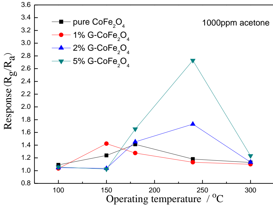
Fig-4: The responses to acetone vapor (1000 ppm) of sensors based on pure CoFe 2 O 4 and G-CoFe 2 O 4 (180°C, 12 h) with different mixing ratio
